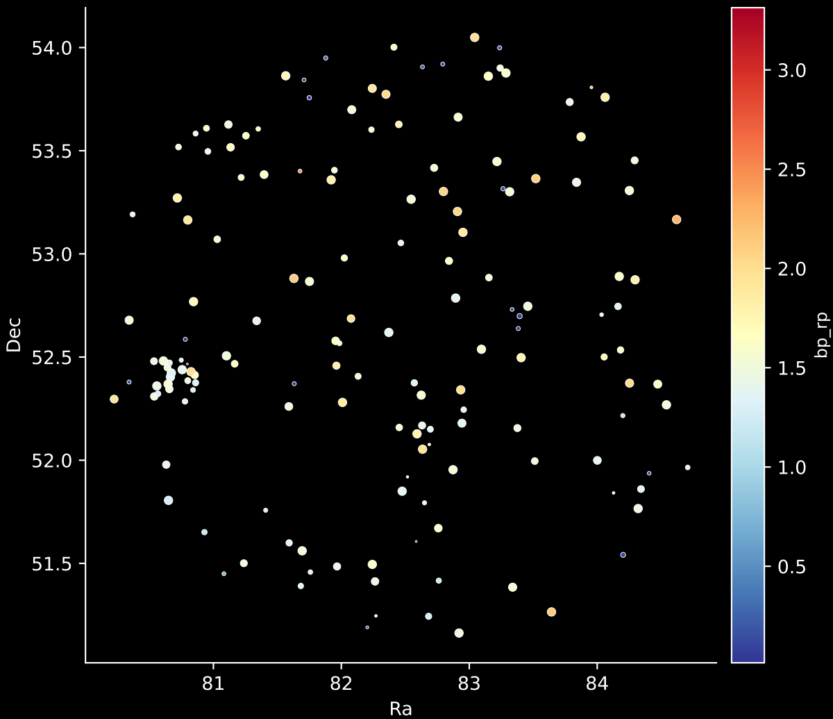
APOGEE DR17 Field: [105-06] Stars: 158
