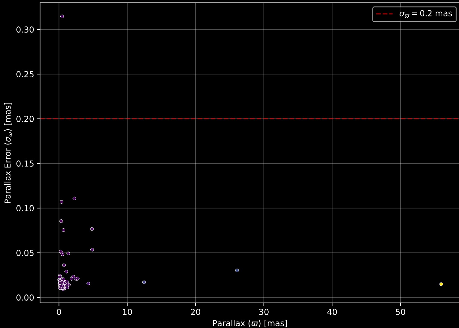
APOGEE DR17 Field: [105-06] Parallax Quality (n= 158)
