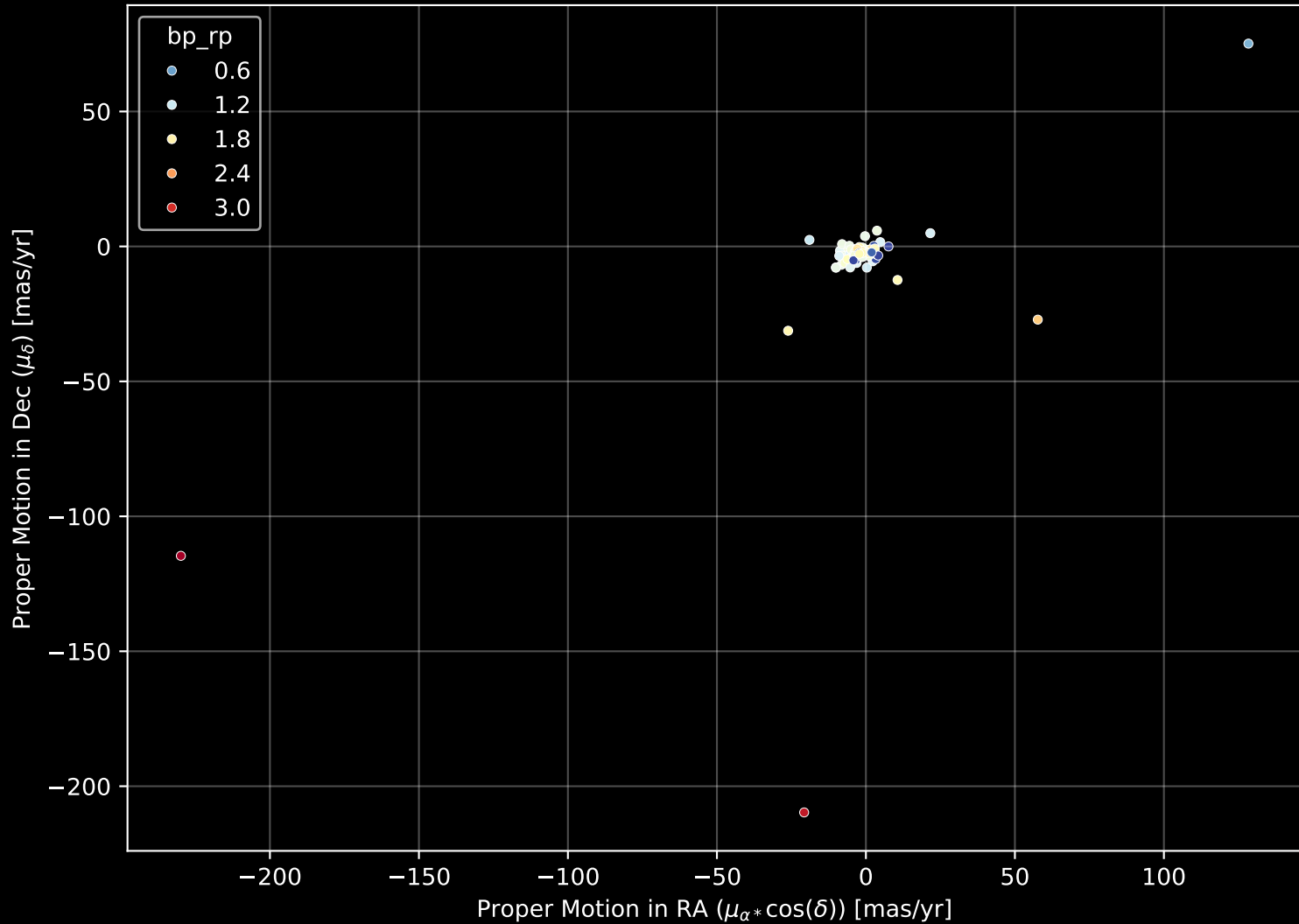
APOGEE DR17 Field: [105-06] Proper Motion Diagram (n= 158)
