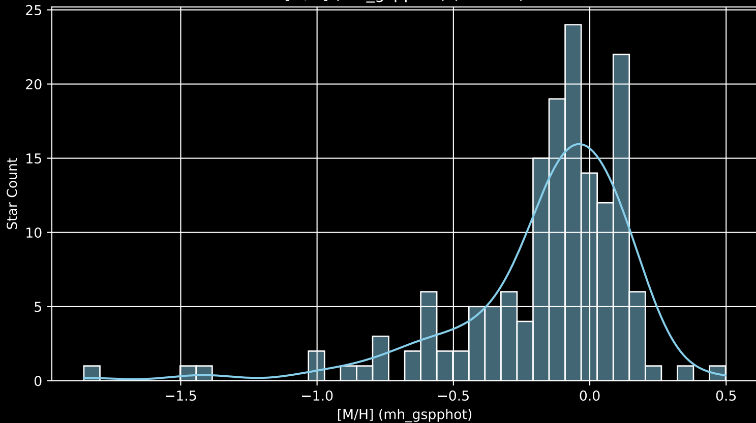
APOGEE DR17 Field: [105-06 [M/H] (mh_gspphot) (n= 157)
