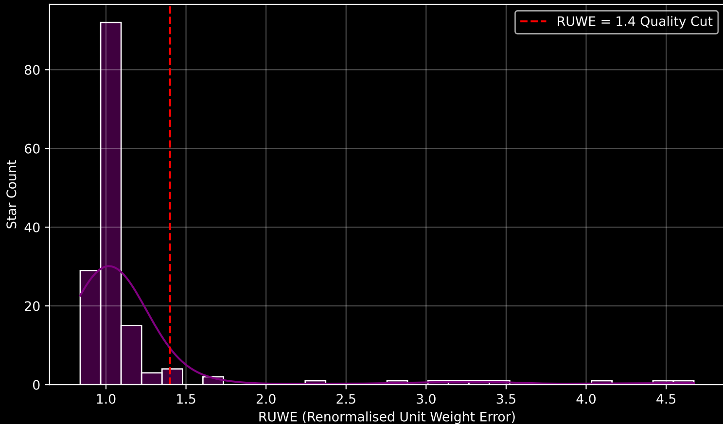
GAPOGEE DR17 Field [105-06] RUWE Distribution (n= 154)
